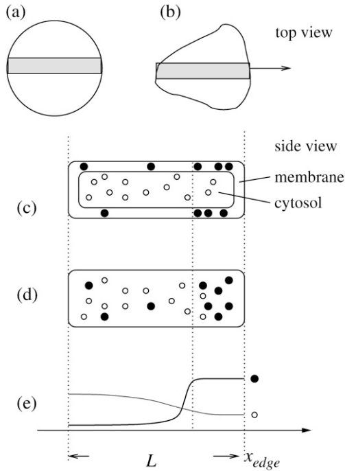
FIGURE 2 Geometry of the model, showing the cell (stationary in panel a , and later motile in panel b ) with a one-dimensional transect (shaded bar), as viewed from the top. (c) ( Enlarged side view ) The transect contains intermediates such as Rho proteins in the membrane (solid disks) and cytosol (open circles) treated as effective concentrations in vertical cross-sections (d), rather than in distinct compartments. Membrane proteins diffuse laterally more slowly than their cytosolic counterparts. As a result, the gradient in cytosolic proteins is much shallower than in the membrane fraction ( thin versus thick lines in panel e ). The axis indicates direction of motion, position of cell edge, and length of the cell. Other intermediates (actin filaments, etc.) are not shown in this schematic. The thickness of the transect has been greatly enlarged for visual clarity, and is neglected in the model.
