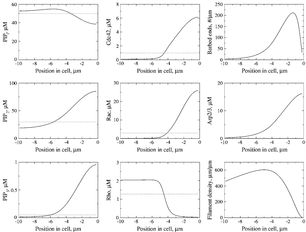
FIGURE 4 (Left column) Spatial profiles of PIs (from top to bottom: \text{PIP}_1 , \text{PIP}_2 , \text{PIP}_3 ); (middle column) Active Rho proteins (Cdc42, Rac, Rho); and (right column) actin (barbed ends, Arp2/3, and filament density) in response to the stimulus described in Fig. 3 a . The spatial profiles are consistent with experimental observations, with \text{PIP}_2 , \text{PIP}_3 , Cdc42, and Rac elevated at the front of the cell and Rho elevated at the rear. The dotted line shows the homogeneous prestimulus distribution (i.e., before a gradient is applied to k_{\text{PI3K}} and k_{\text{PTEN}} ), while the solid line shows the post-stimulus steady-state distribution. The leading edge of the cell is on the right in each frame.
