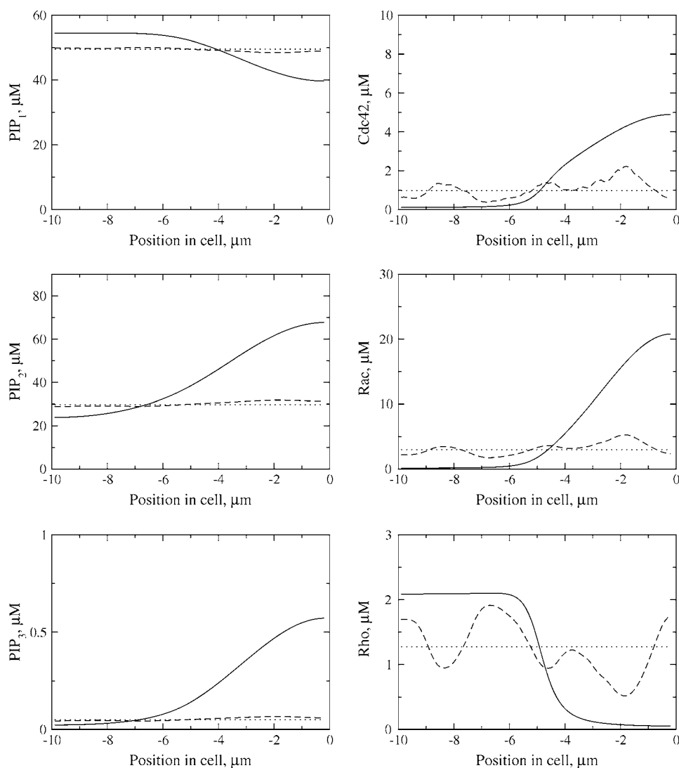
FIGURE 8 PIs act to smooth out Rho proteins and prevent establishment of multiple domains of high Cdc42 in response to a random stimulus (compare with Fig. 7). Spatial profiles are shown before ( dotted line ), during ( dashed line ), and 50 s after ( solid line ) application of the stimulus. Upstream regulation of the Rho proteins by PIs ensures the establishment of a single domain with high Cdc42 at the front of the cell when the cell is exposed to a random stimulus (in contrast to Fig. 7).
